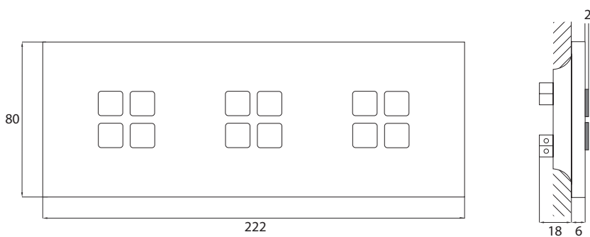
H142 222X80X6
