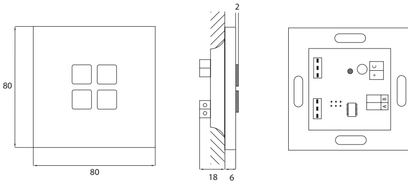
502 80x80x6
