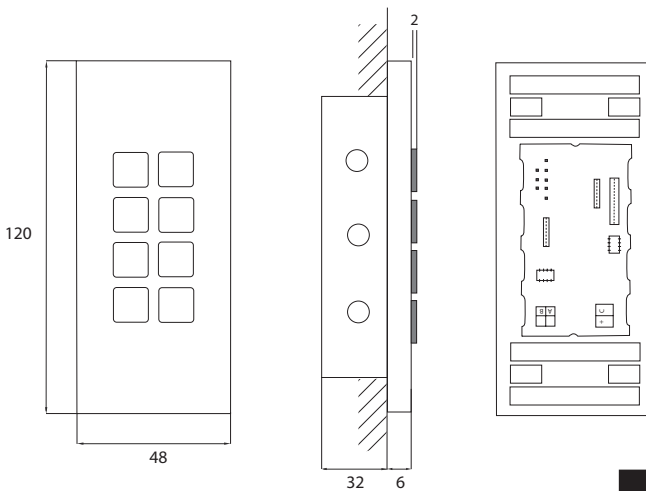
503 SLIM 120x48x6
