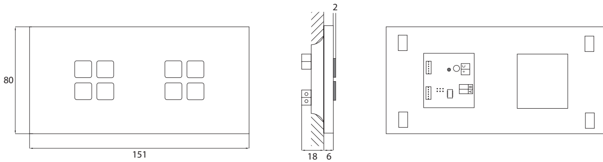
H71 151X80X6
