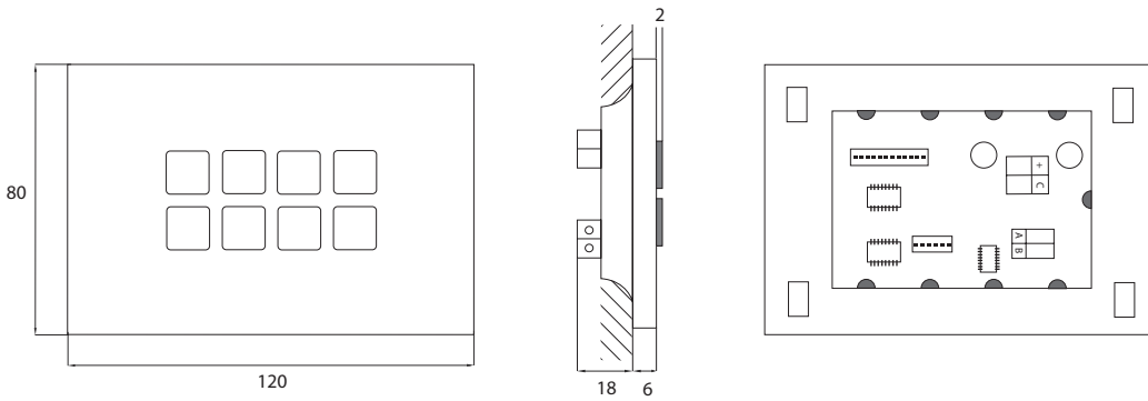
503 120x80x6
